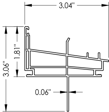
6 SILL
