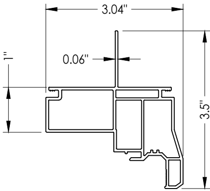
1 FRAME HEAD
