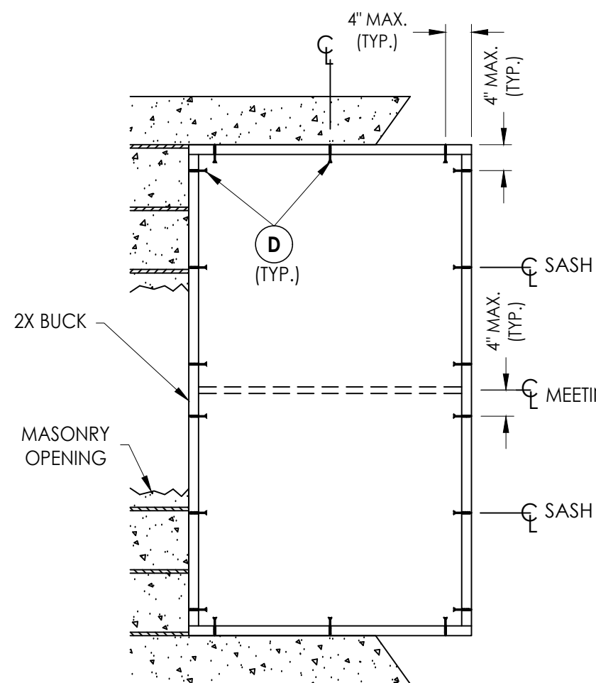
BUCK ANCHORING
