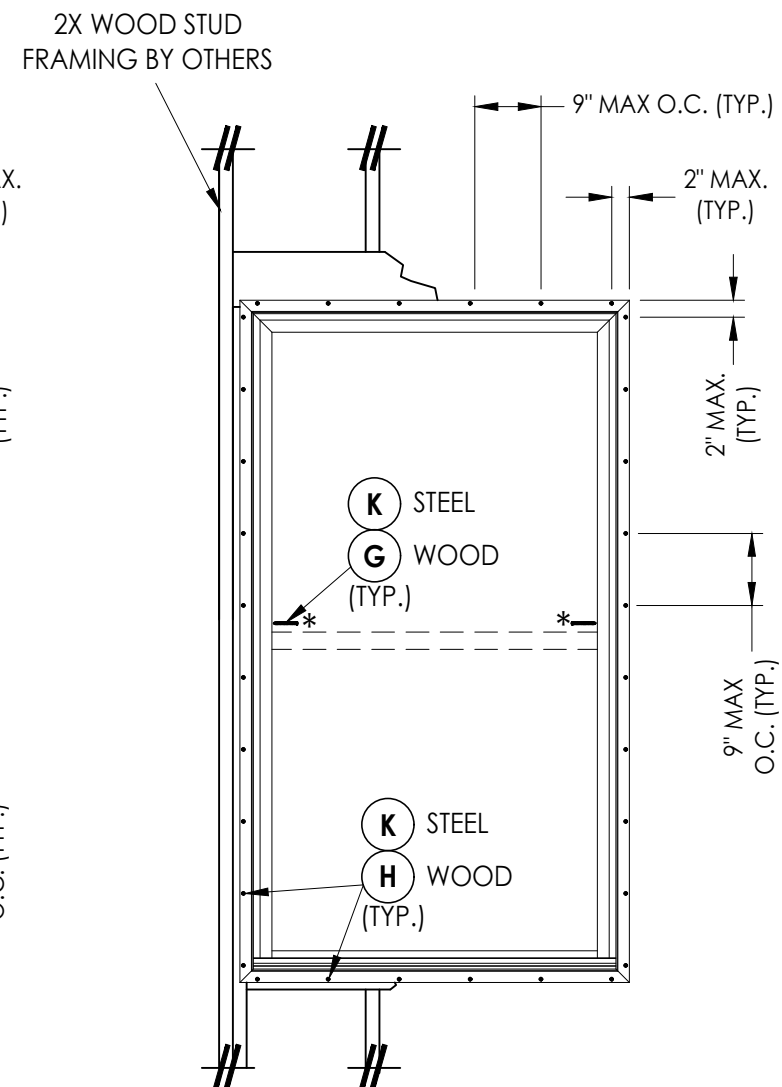
FRAME ANCHORING
